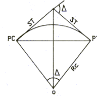
Curva circular simple
